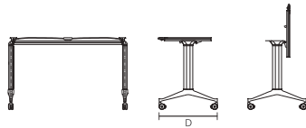
Metal Frame Dimension L=1140-1740mm D=580mm H=725mm
